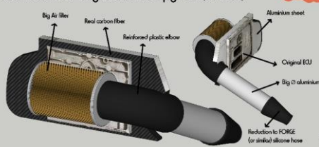
Smart Roadster - High Airflow Kit Upgrade (RENDER)
